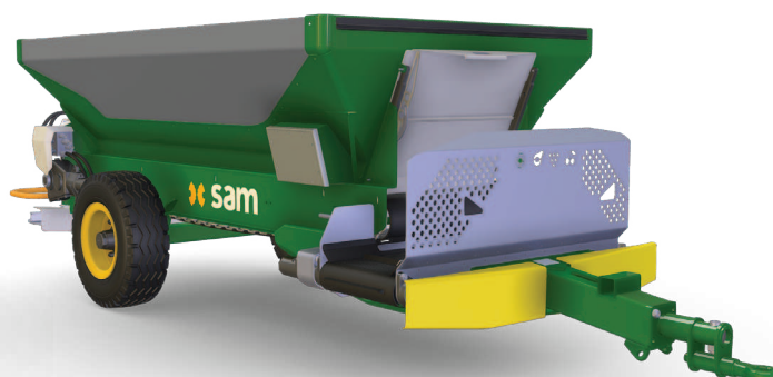
Front view showing banding conveyor
